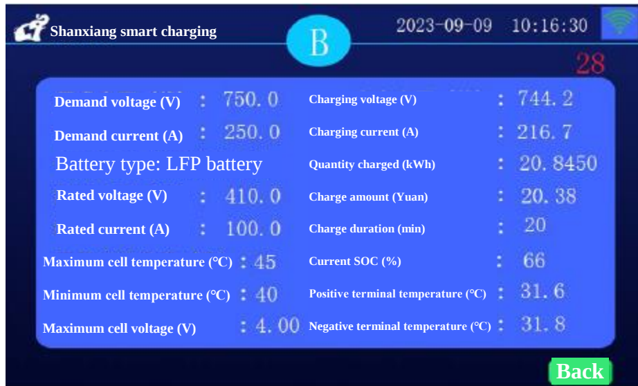
Charging Process Data Display Figure
