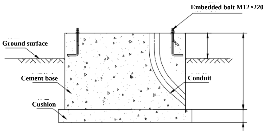
Charger Foundation Drawing
