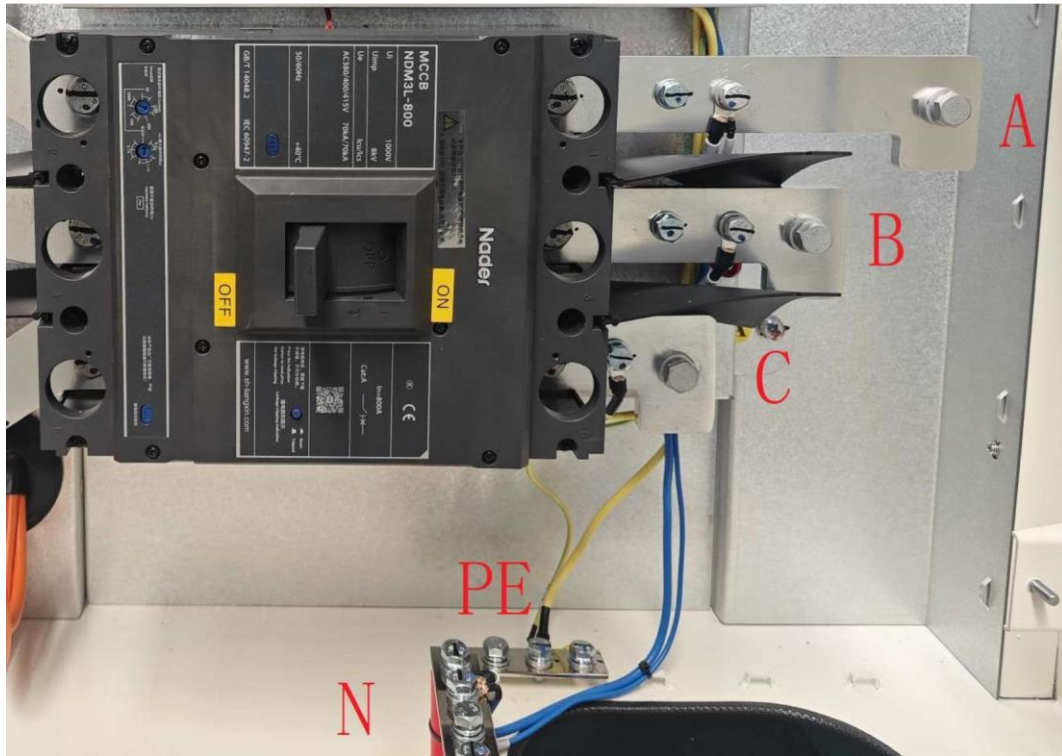
AC charging input cable installation position figure
