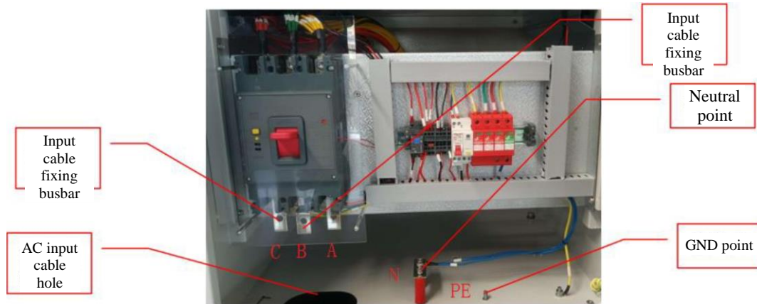
AC charging input cable installation position figure
